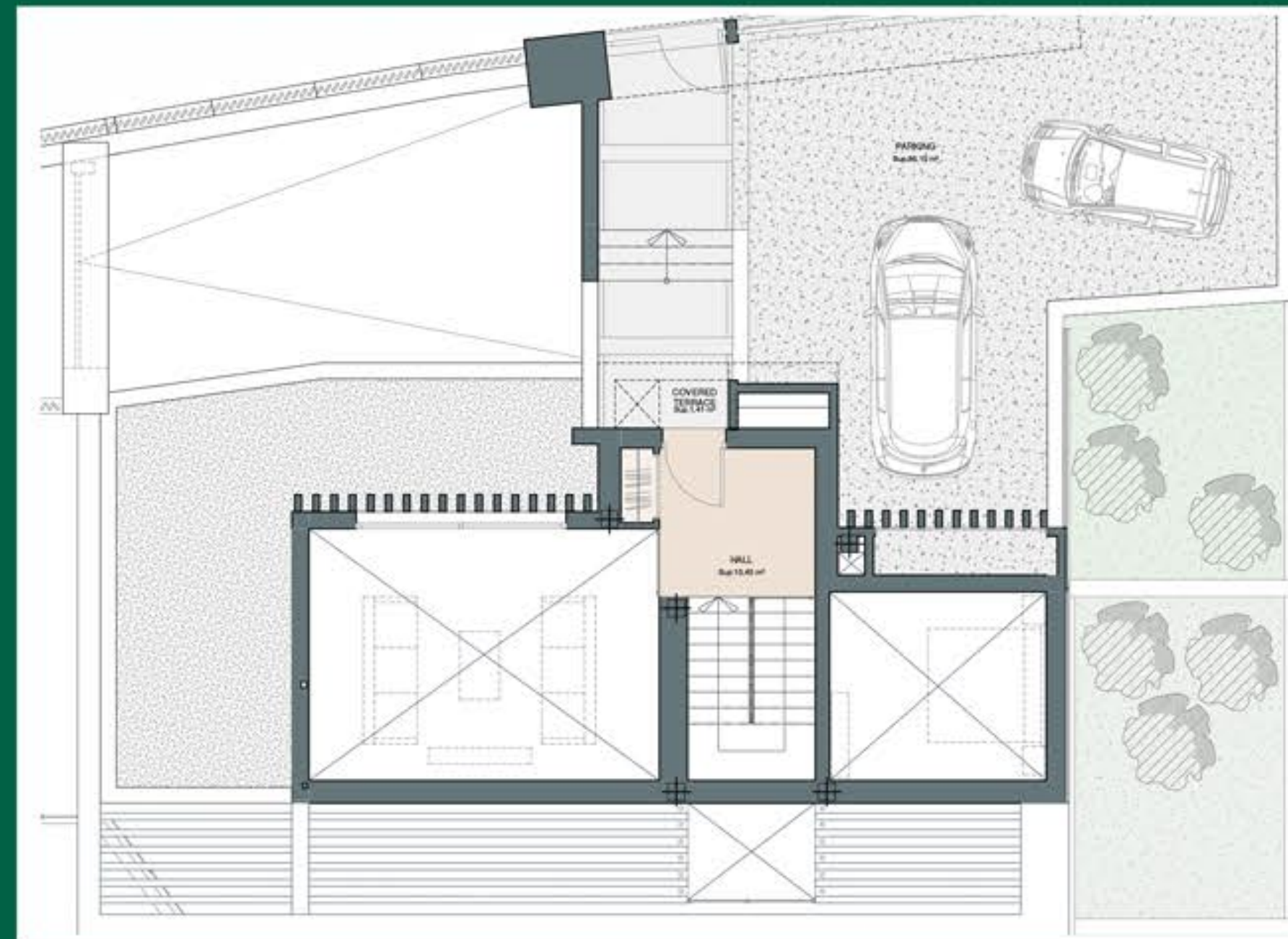
ENTRANCE FLOOR
