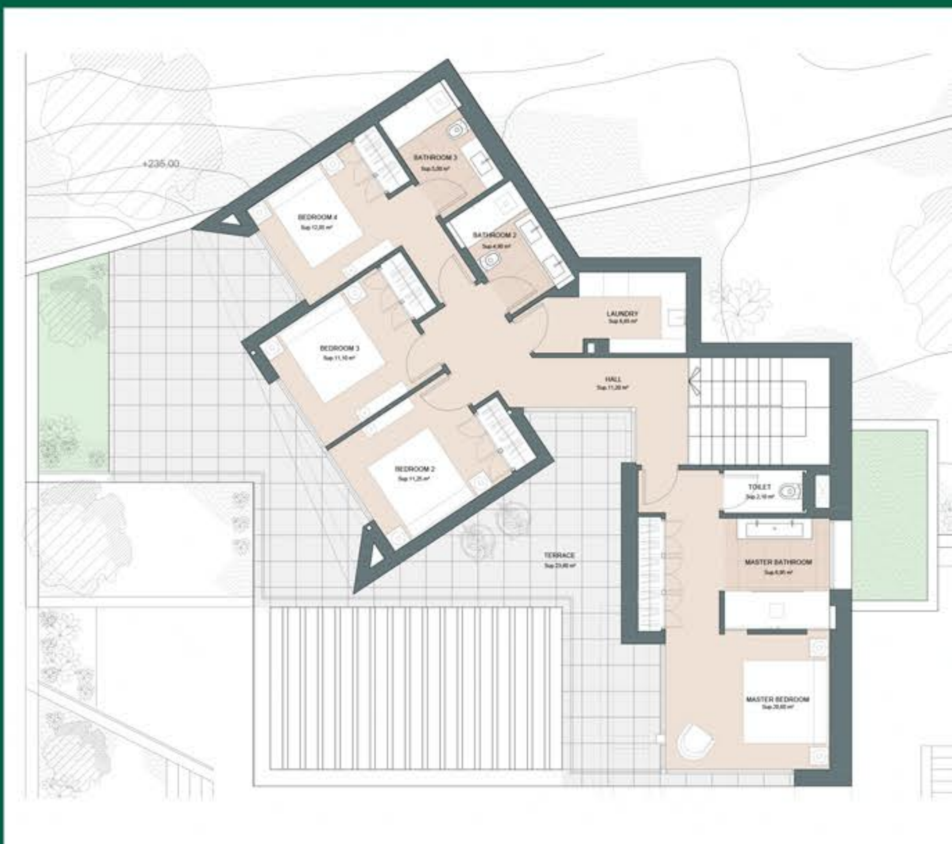
FIRST FLOOR
