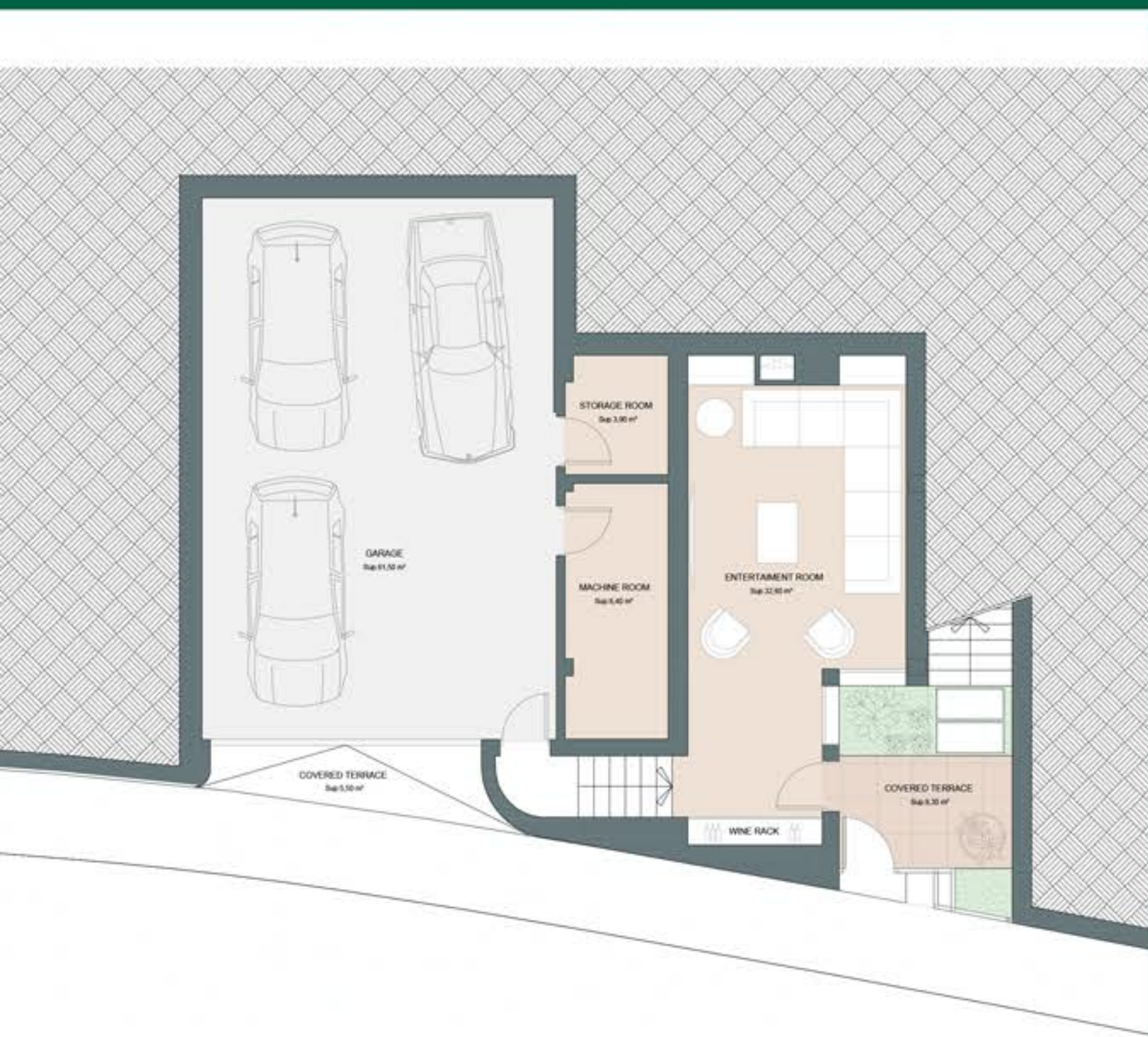
BASEMENT
