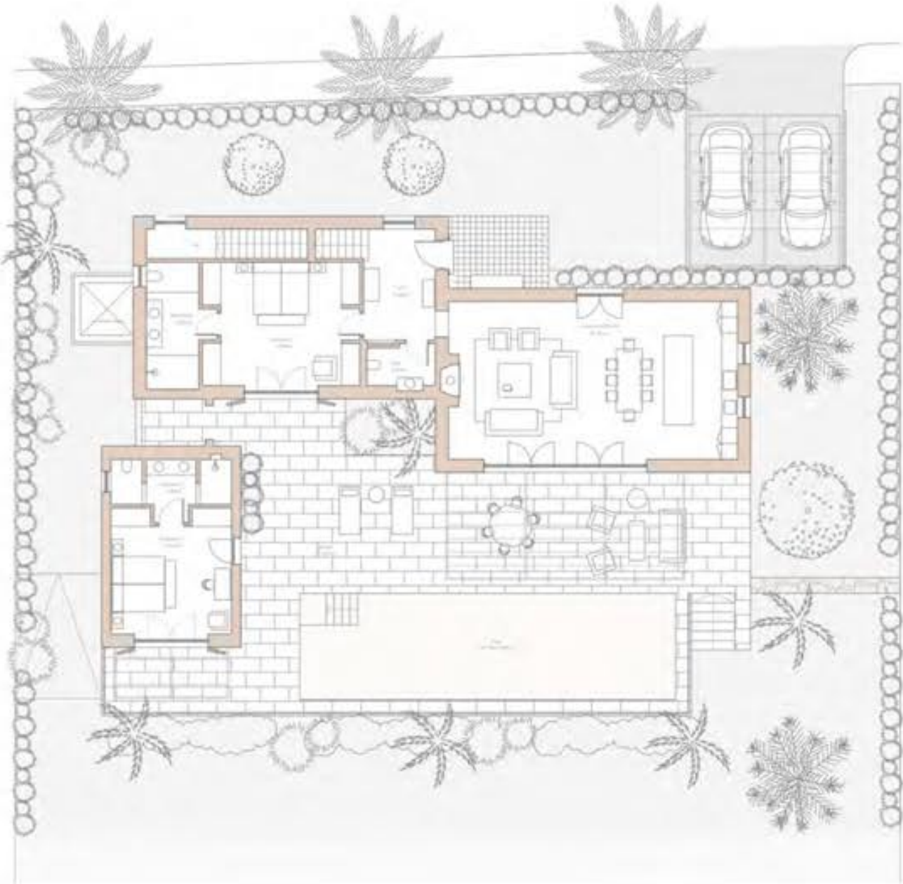
Planta Baja Ground Floor
