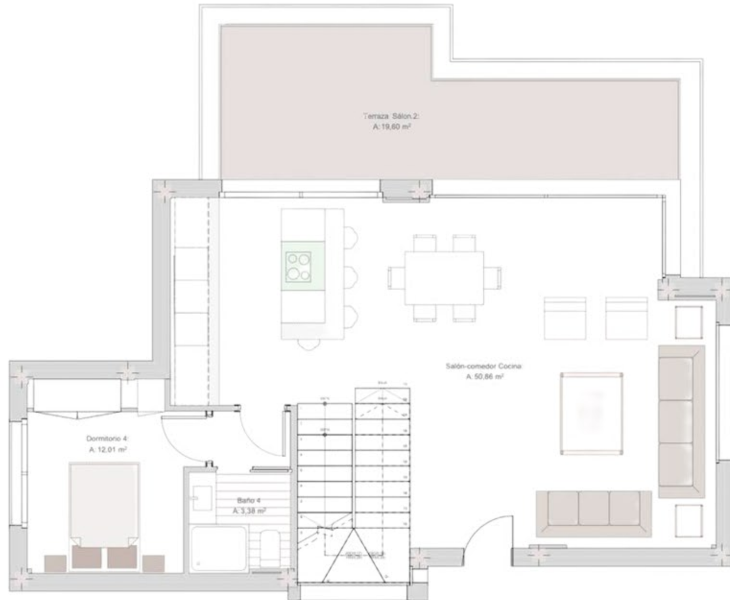
GROUND FLOOR
